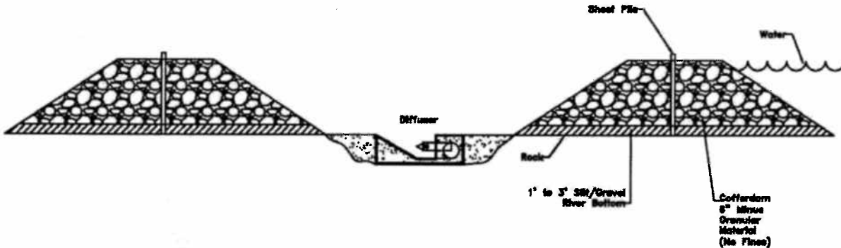
Figure 6. Proposed Cofferdam Cross Section.
