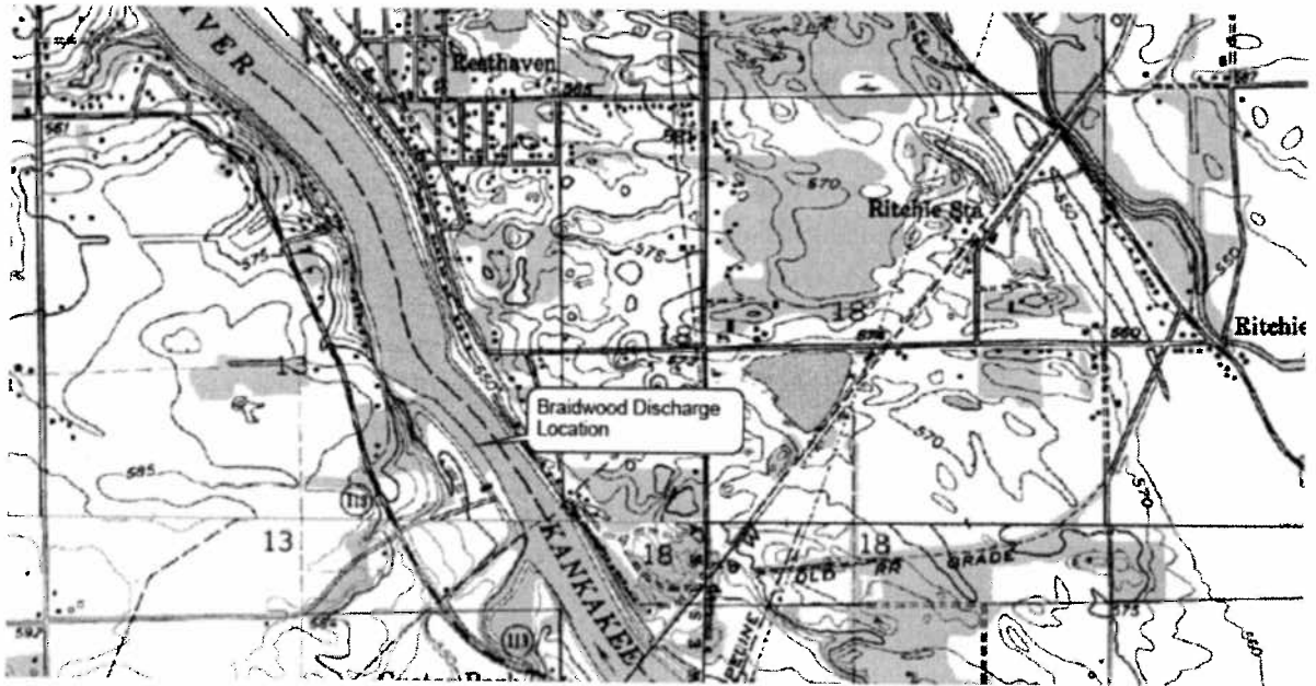
Figure 2. Braidwood River Diffuser Discharge Location Topo Map.
