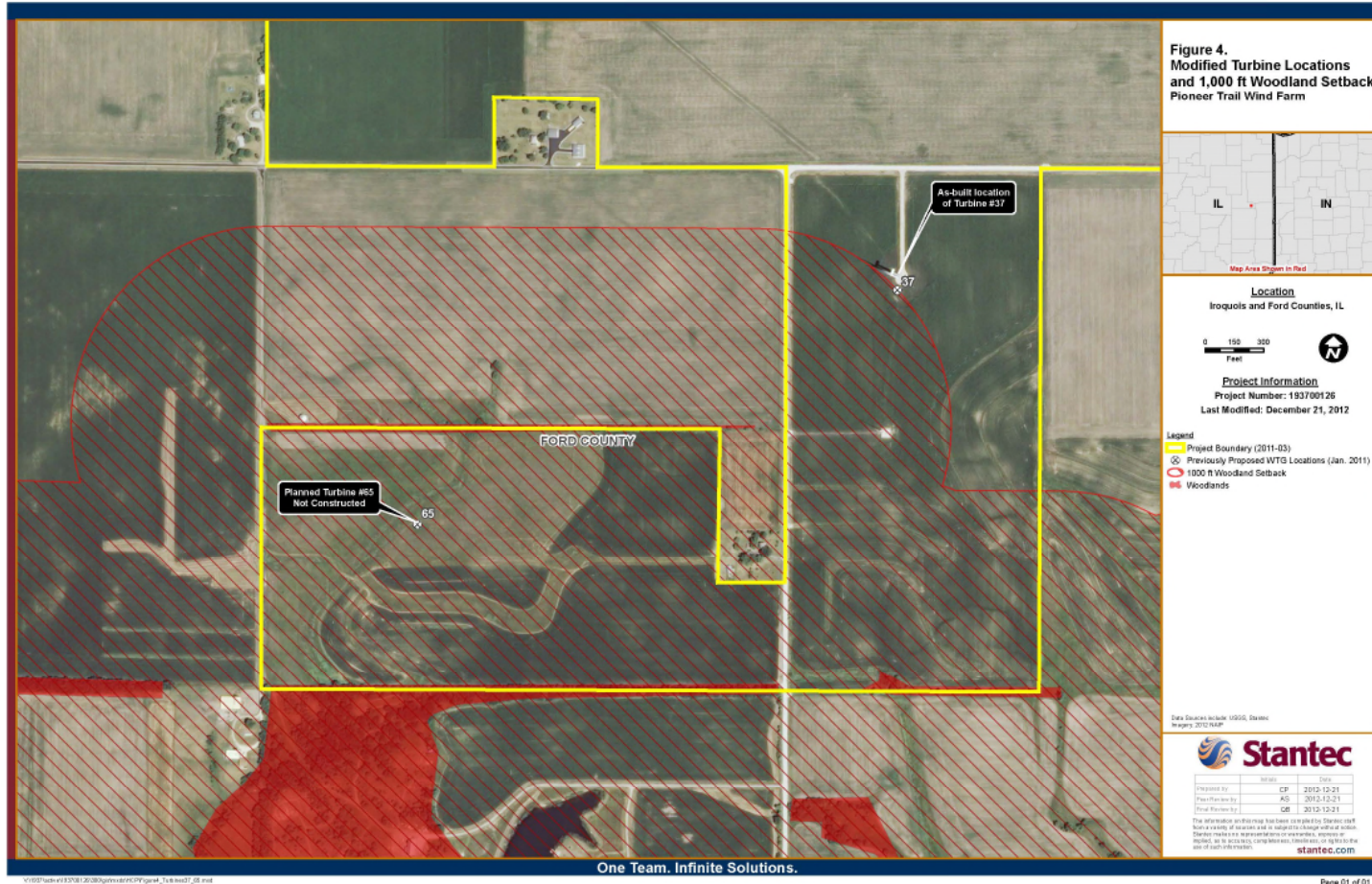
Figure 4. Modified Turbine Locations and 1,000 foot Woodland Setback
